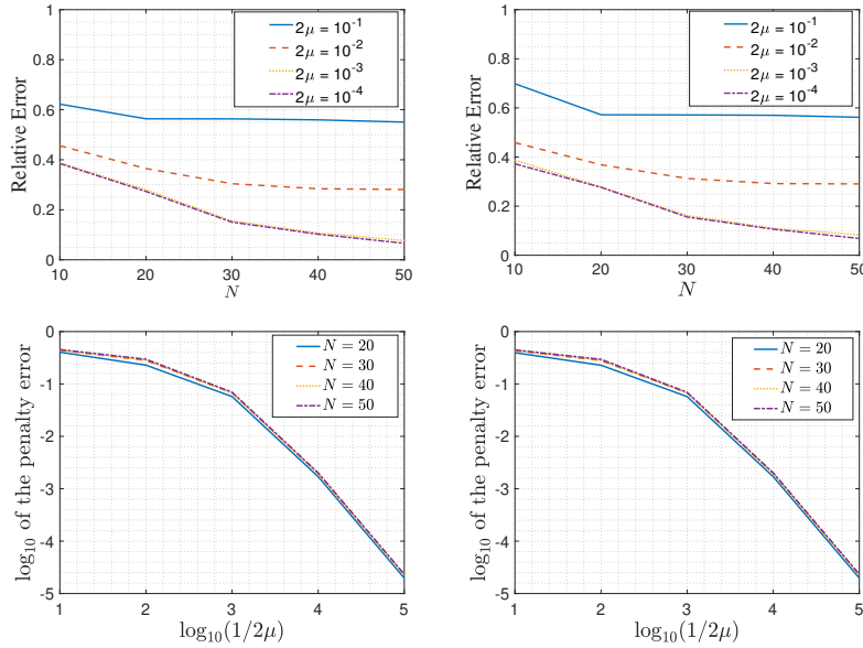
Figure 2: The relative error \|D_{\mu, N} - D_{\text{exact}}\|_{L^2(\Omega)} / \|D_{\text{exact}}\|_{L^2(\Omega)} vs. N for several \mu -values (Top) and the penalty error \text{PE}(\mu, N) vs. 1/(2\mu) for several values of N (Bottom) for B(s) = s^2/2 (left) and B(s) = \cosh(s) - 1 (right).
